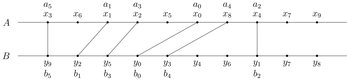
Figure 6.1: The order-isomorphism between \mathfrak{A} and \mathfrak{B} constructed in Theorem 6.14.
