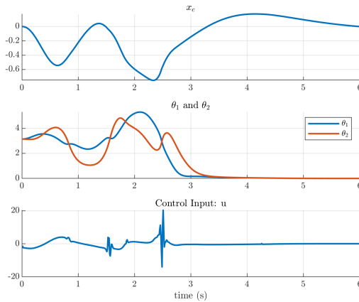
Fig. 5. Positions, input vs time
