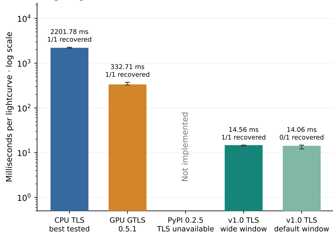
Single lightcurve
