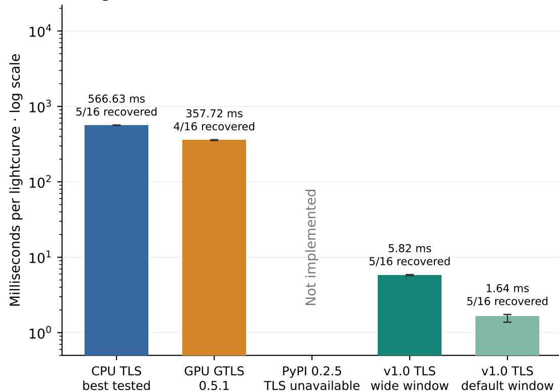
16-lightcurve workload
