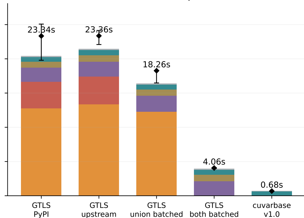
Rubin-like: 313,007 periods
