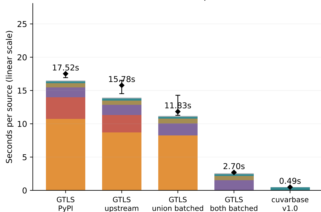
ZTF-like: 219,127 periods
