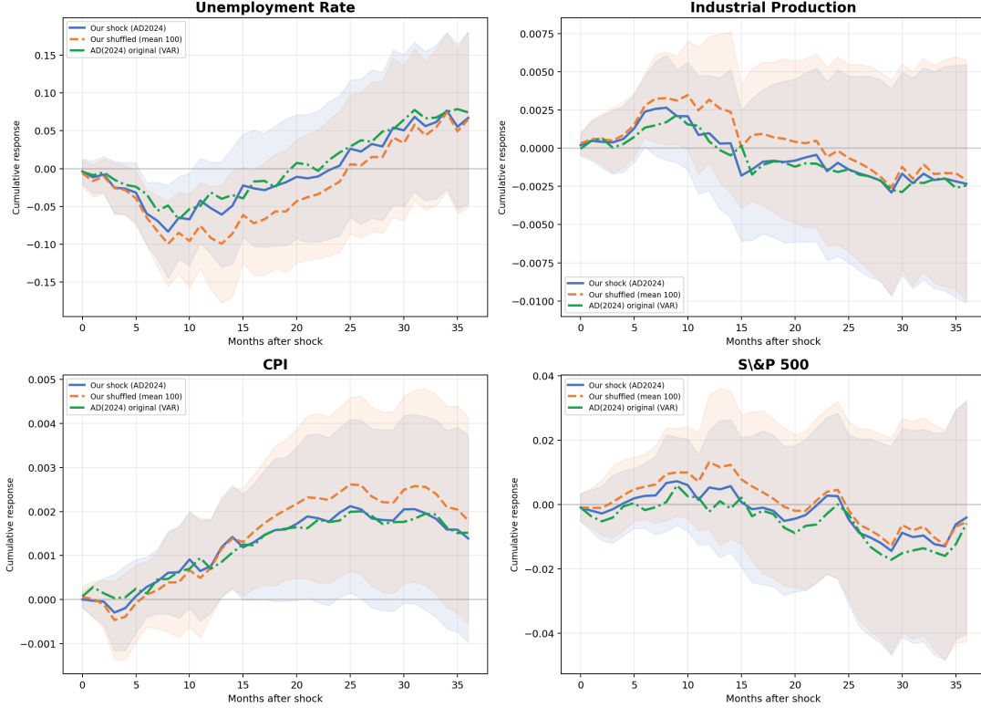
Figure 1: Cumulative IRF ( y_{t+h} - y_{t-1} ) to a one-standard-deviation monetary shock. Our replication shock (blue), mean shuffled shock (orange), and AD(2024) original VAR shock (green). Confidence bands (95%) shown for our two shocks. The IRFs start at h = 0 (contemporaneous response) and evolve from there.
