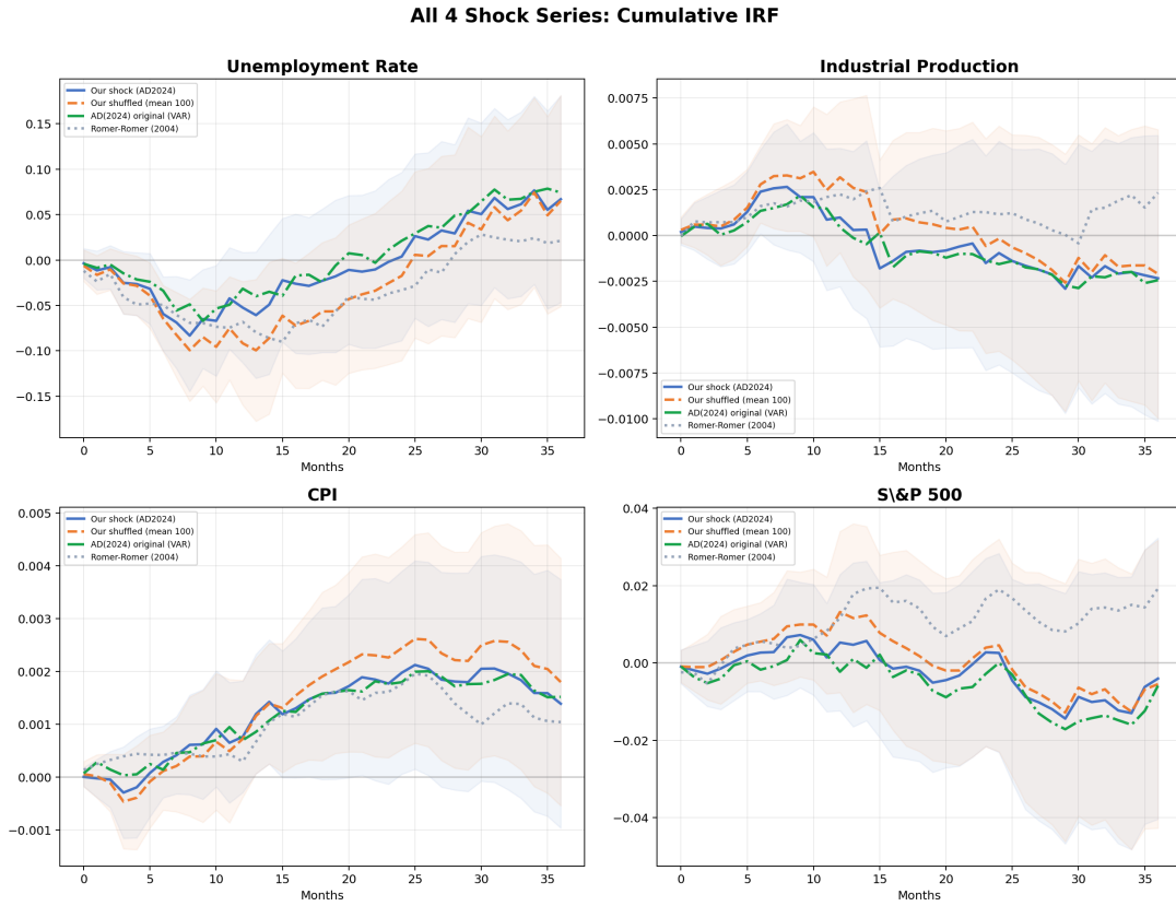
Figure 2: All four shock series: cumulative IRF comparison. Romer-Romer shock (gray, dotted) has fewer non-zero months, producing wider effective dispersion.
