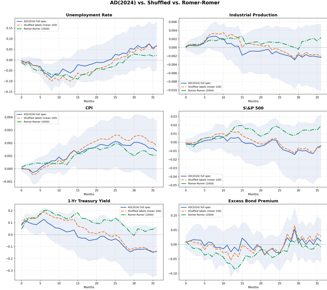
Figure 1: Cumulative IRF for six macro variables. AD(2024) full spec (blue, solid, with 95% CI), shuffled labels (orange, dashed), and Romer-Romer 2004 (green, dash-dot).
