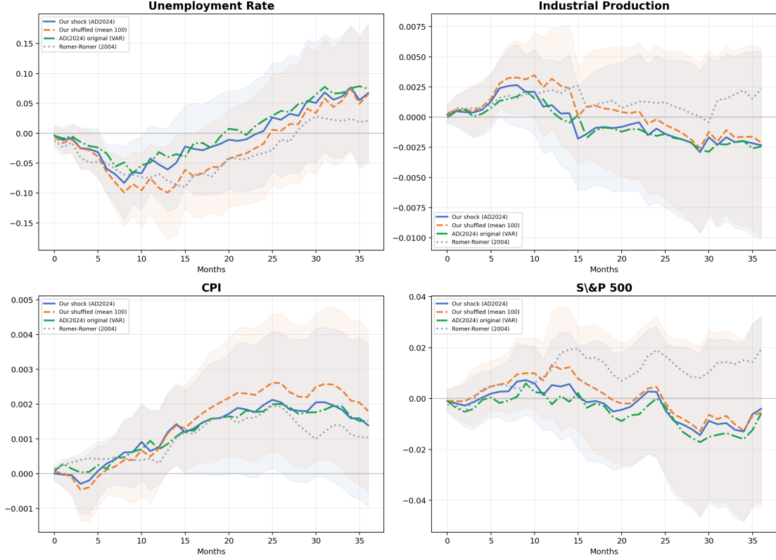
Figure 2: All four shock series. Romer-Romer (gray, dotted) has fewer non-zero months (only FOMC meeting months), producing wider effective dispersion and less precise IRF estimates.
