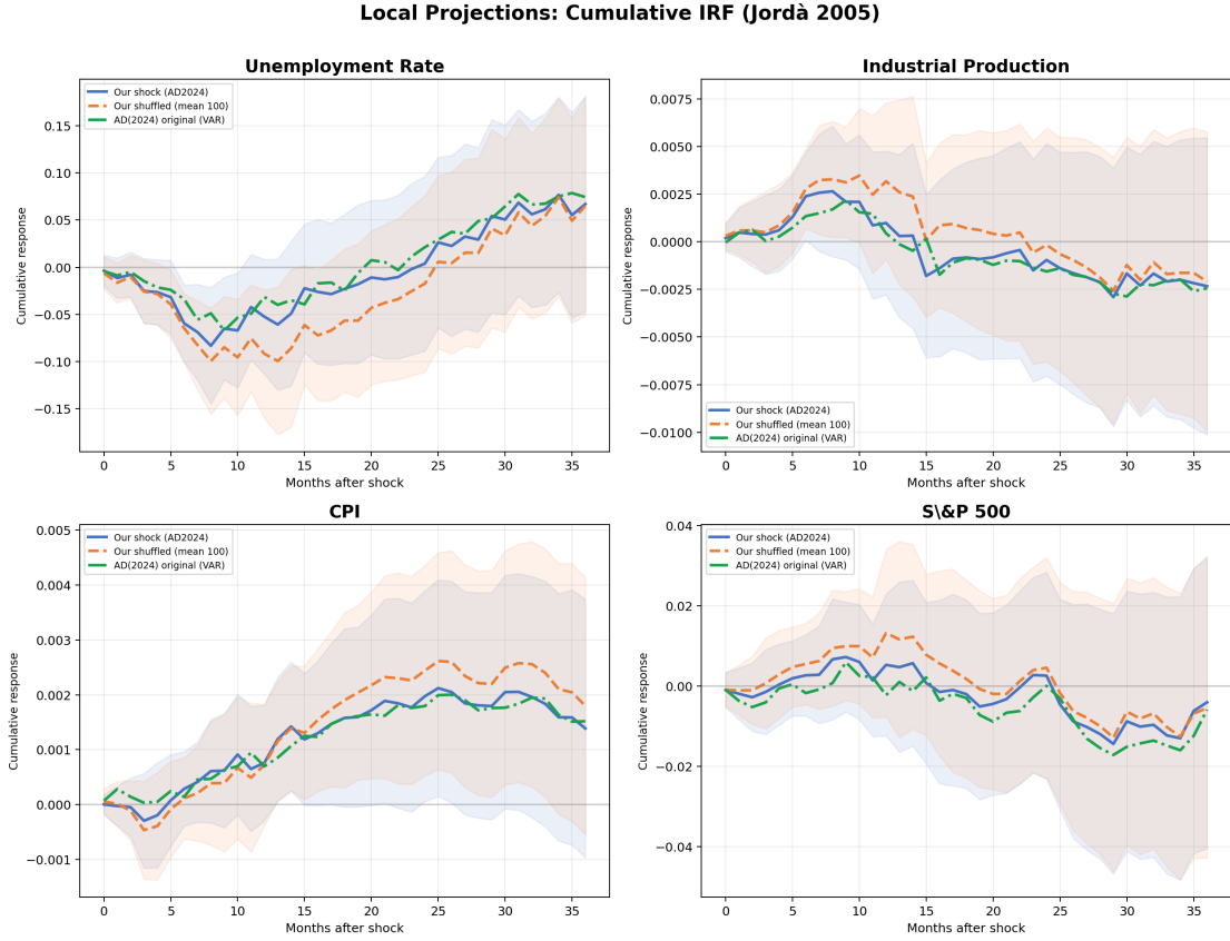
Figure 1: Cumulative IRF: our replication shock (blue, solid), mean shuffled shock (orange, dashed), and AD(2024) original VAR shock (green, dash-dot). 95% confidence bands for our two shocks.
