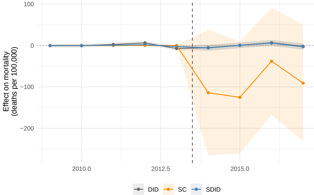
Figure 2: Event-study comparison across estimators.
