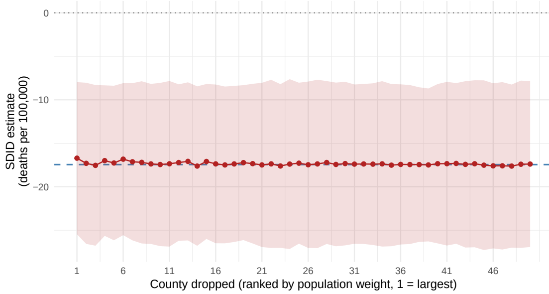
Figure 4: Leave-one-out sensitivity of the population-weighted SDID estimate.
