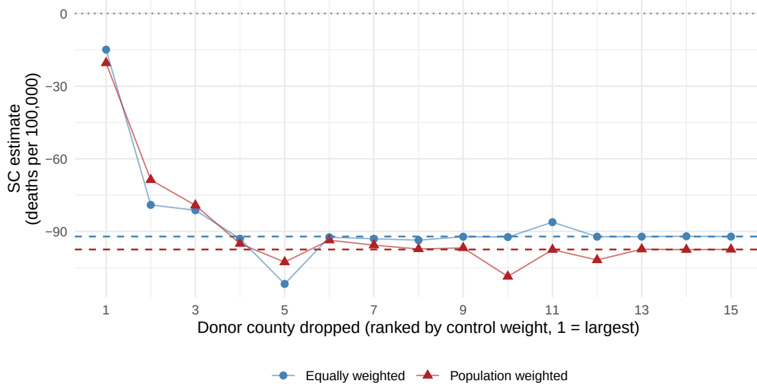
Figure 1: Leave-one-out donor sensitivity of the SC estimates.
