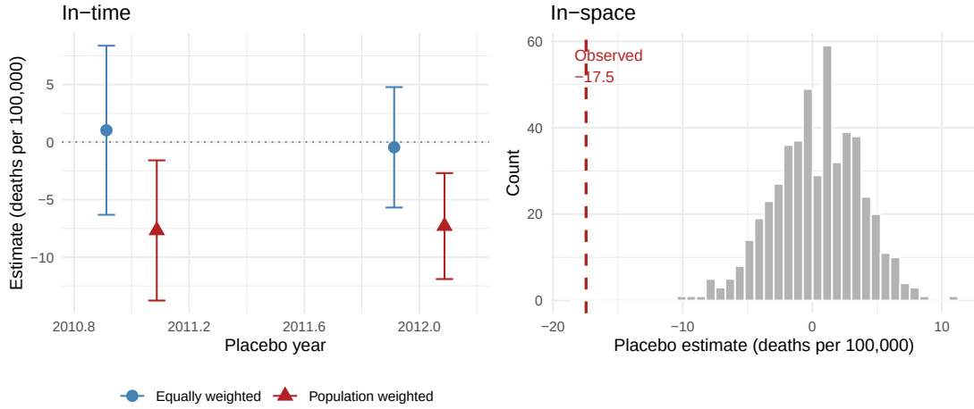
Figure 4: Placebo tests.
