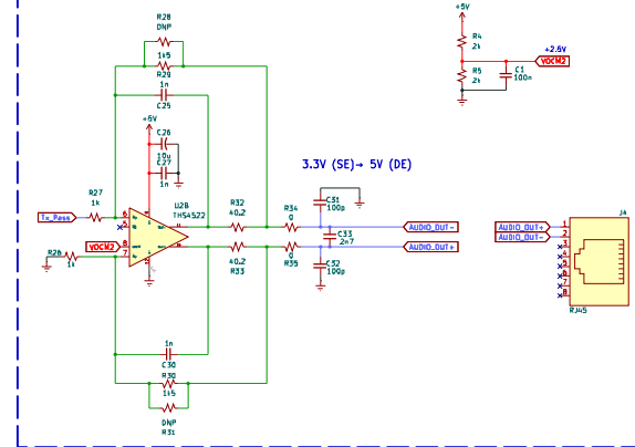
AES3 Differential Output Driver
