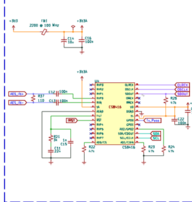
Digital Audio Receiver (AES3 → I2S)
