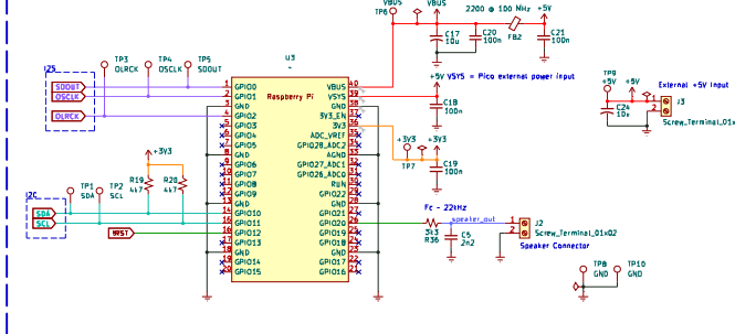
Raspberry Pi Pico
