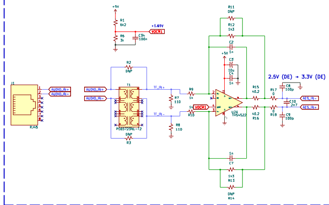
AES3 Differential Input Front-End
