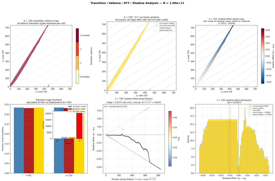
Figure 7. Transition and shadow analysis at k = 729 , N = 10^{11} . Top left: Transition valence map, each non-empty cell is colored by the number of distinct transition types (ee, eo, oe) it exhibits; the ghost island appears as a secondary band near r_3 \approx 440-460 . Top center: "11" successor analysis verifying the golden mean shift at each cell. Top right: Shadow offset spatial map, red cells are closer to the rational foliation 460/729, blue cells closer to the irrational foliation \log_2 3 . Bottom right: Shadow offset distribution with gap near zero and asymmetric shoulder at +0.007 from the ghost island..
