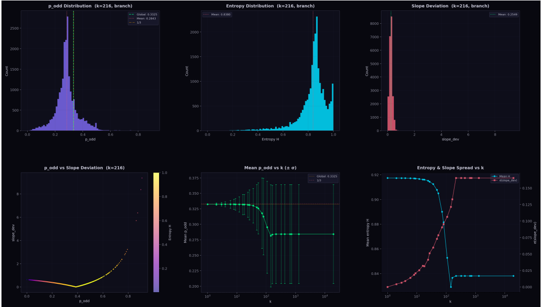
Figure 2. Cell-level statistics at k = 216 . (a) p_{\text{odd}} histogram for branch cells: peaks near 0.28, with the global mean 0.3325 and 1/3 marked. (b) Entropy histogram: most branch cells have H \approx 0.84 , indicating robust even/odd mixing. (d) Scatter of p_{\text{odd}} vs. slope deviation, colored by entropy: a sharp V-shaped cusp at p^* = 1/(1 + \log_2 3) \approx 0.387 , the equilibrium at which the multiplicative drift (3/2)^{v_3} \cdot (1/2)^{v_2} is neutral. The cusp appears at every k -level from k = 9 onward. Most branch cells sit to the left of the cusp ( \bar{p}_{\text{odd}} = 0.284 < p^* ), on the convergent side. (e) Mean p_{\text{odd}} vs. k : stabilizes at 0.284 for k \geq 216 .
