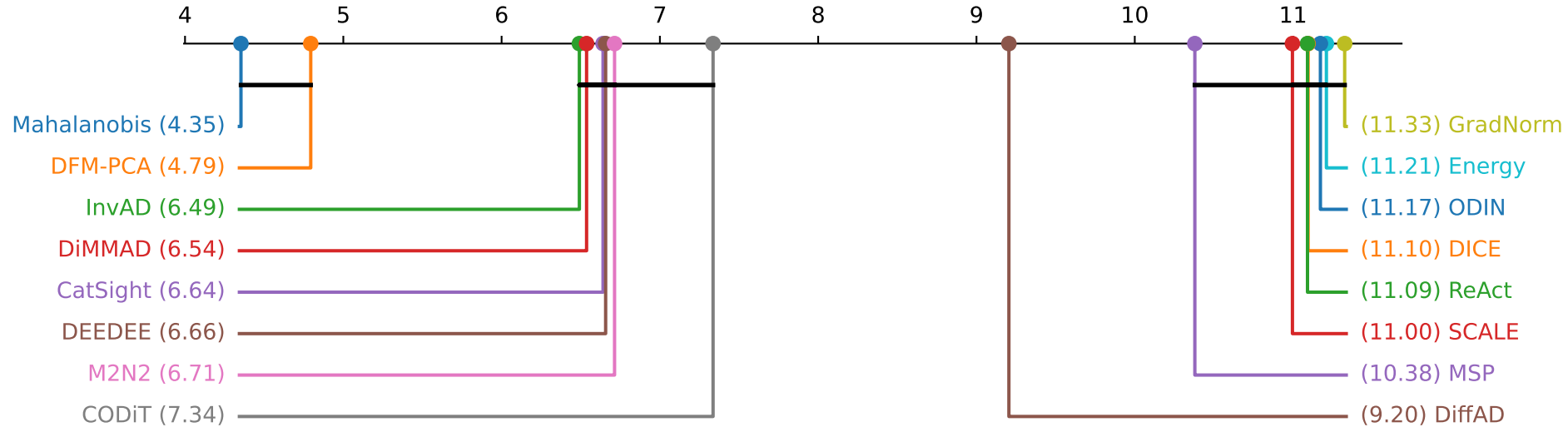
Critical-difference diagram (Nemenyi, \alpha = 0.05 ): 16 detectors, N = 515 datasets, CD = 1.016
