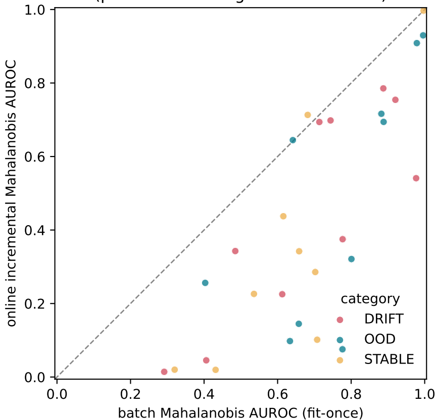
Per-window AUROC on the ordered stream (points above diagonal: online wins)
