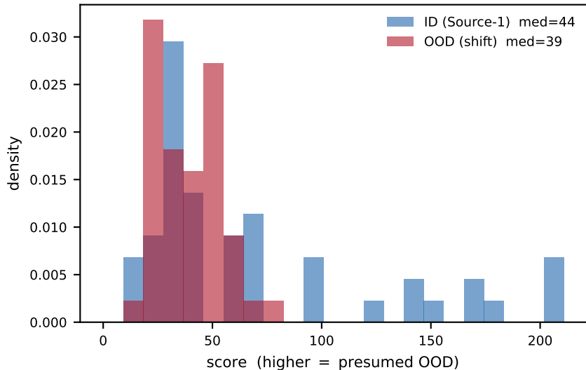
Mahalanobis (feature distance) AUROC = 0.350 [inverted]
