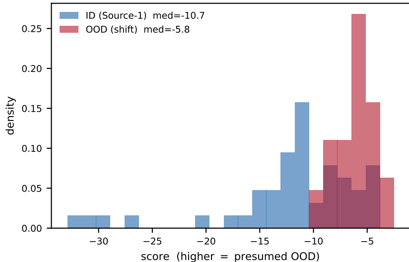
Energy (post-hoc logit) AUROC = 0.852 [correct]
