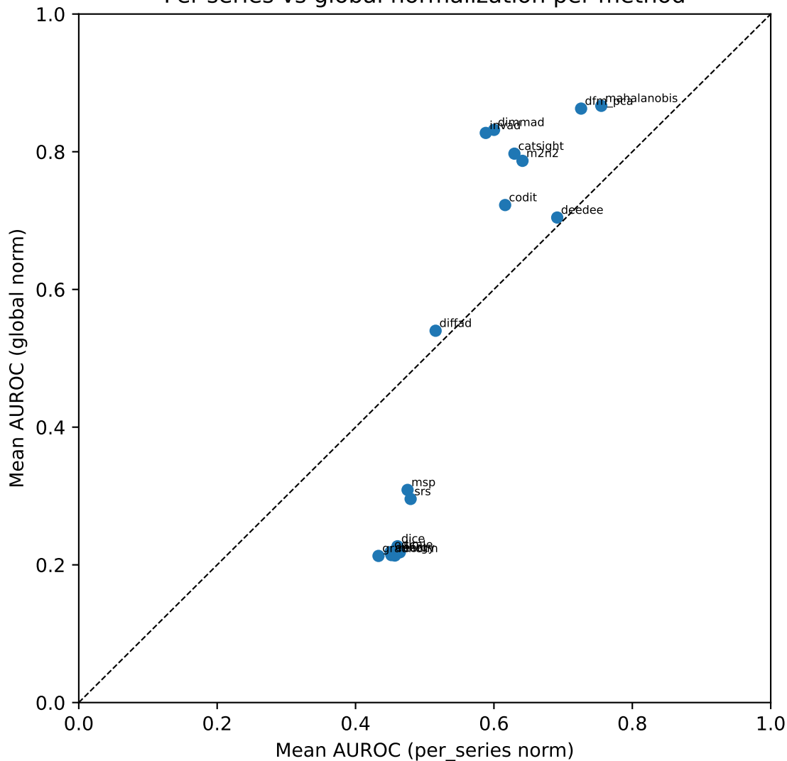
Per-series vs global normalization per method
