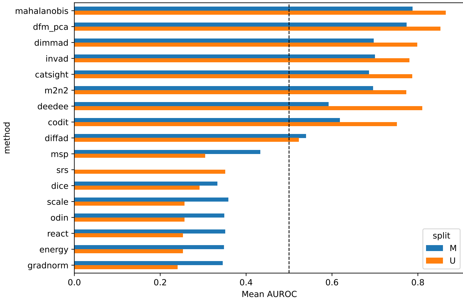
Mean AUROC by method and split (U vs M)
