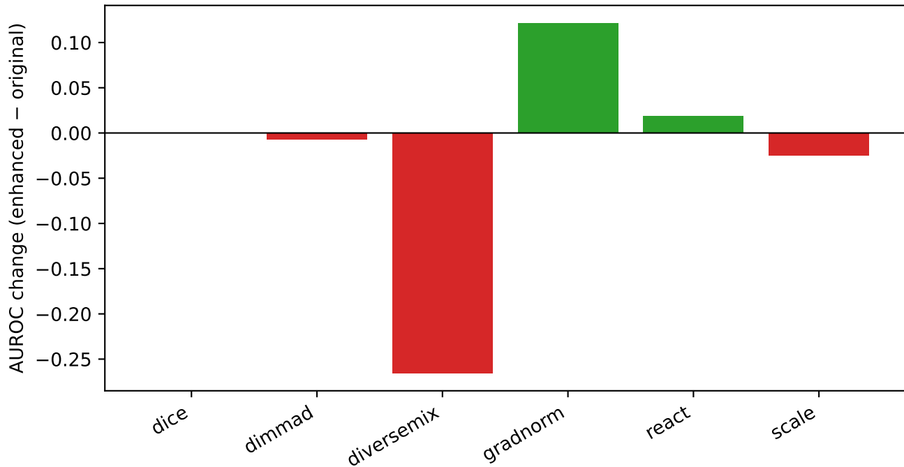
Effect of paper-faithful corrections (mean over datasets)
