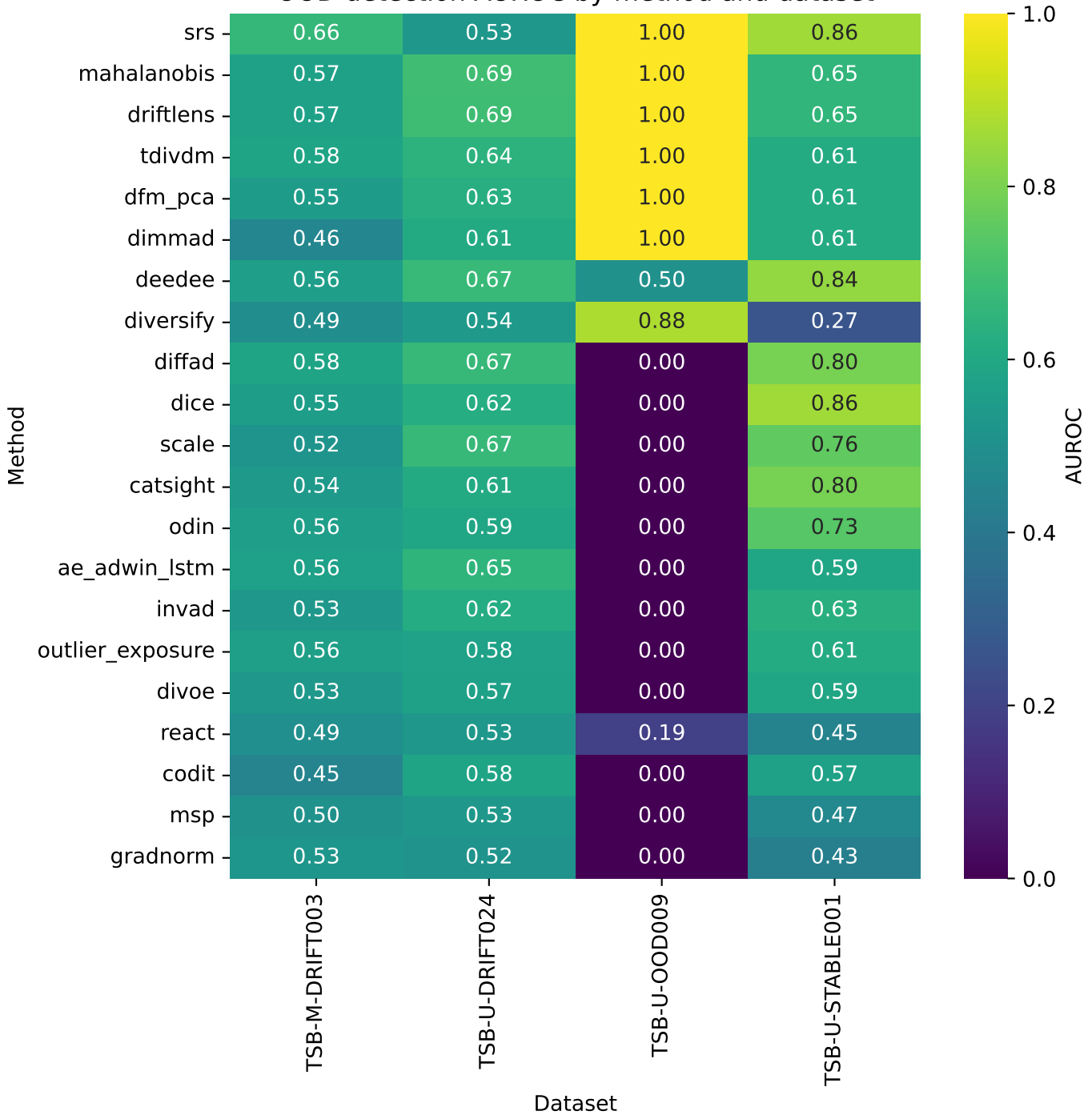
OOD detection AUROC by method and dataset
