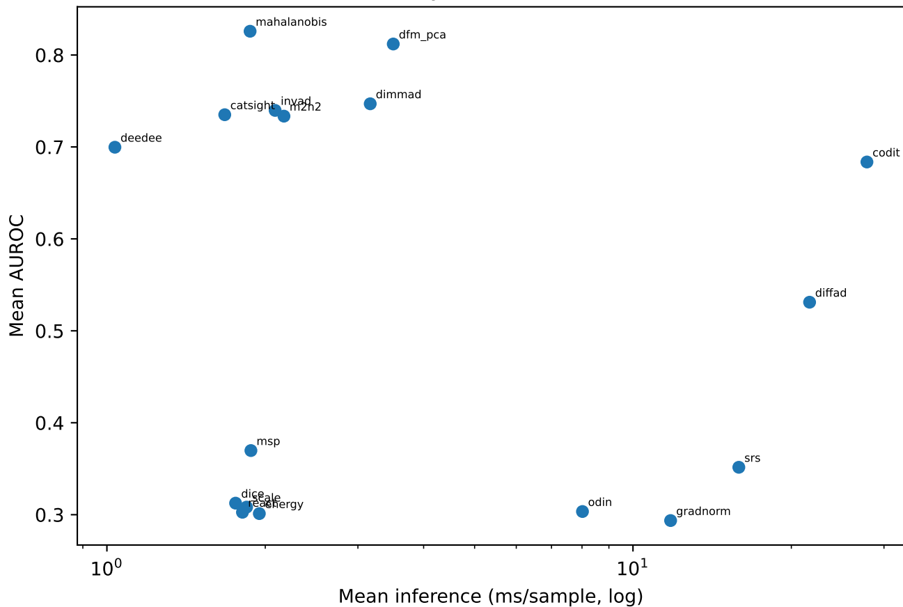
Accuracy vs inference cost
