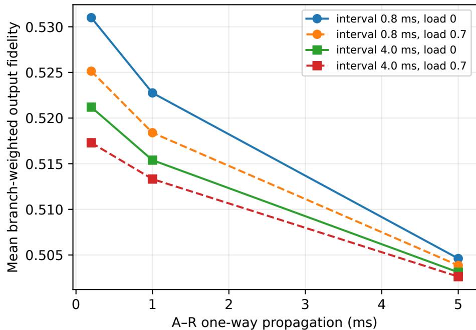
Finite characterization: 4 chains \times 4 traffic phases per condition
