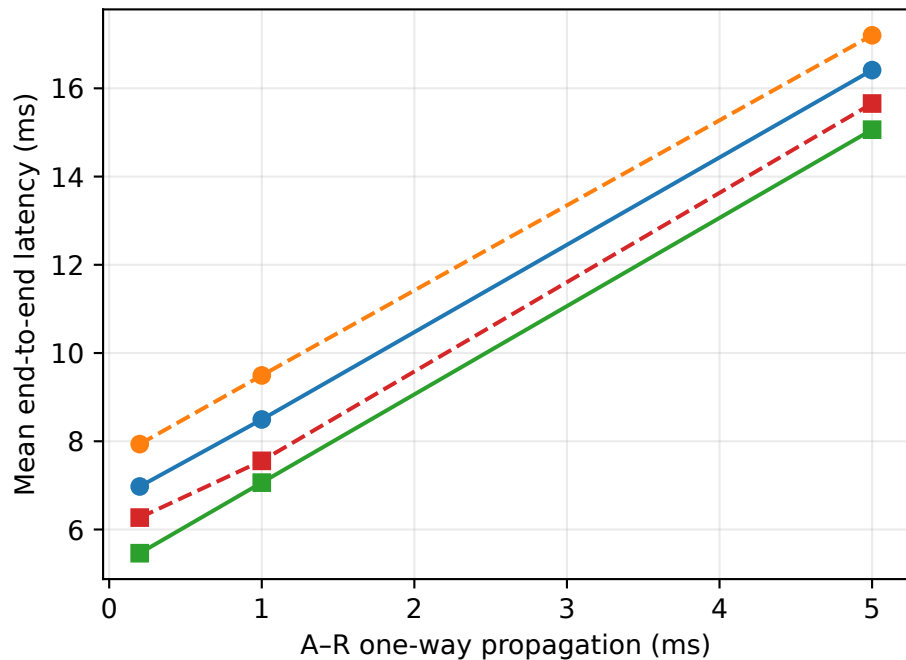
Finite characterization: 4 chains \times 4 traffic phases per condition
