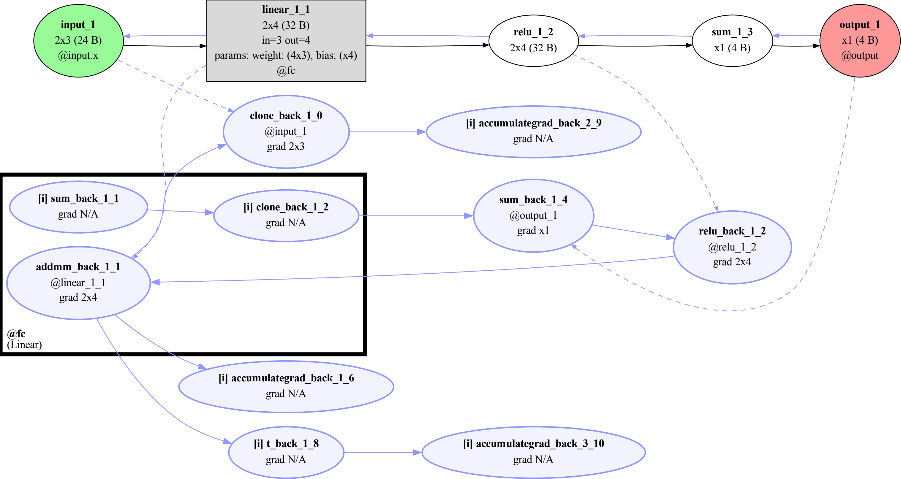
LinearReluModel combined forward/backward graph 5 forward nodes, 10 grad_fn nodes 1 backward pass(es)
