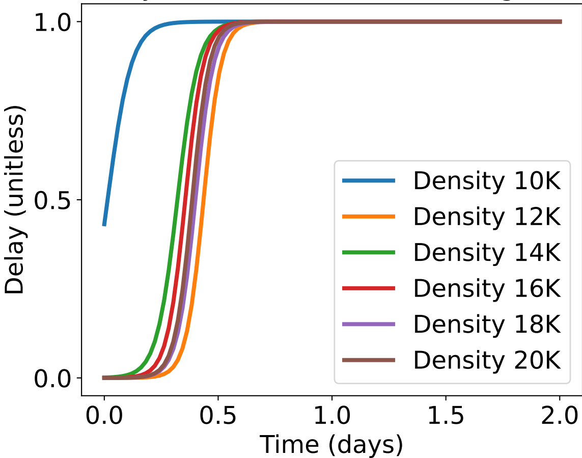
Delay estimates for Wound healing data
