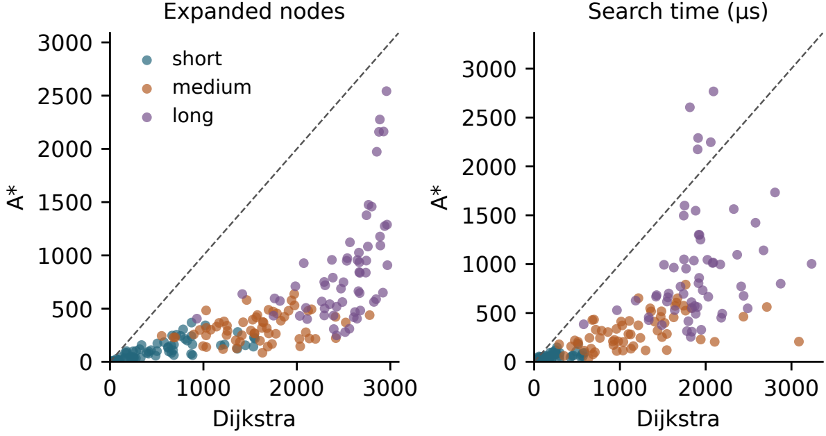
Figure 3: Matched road search effort and search-call timing. Points below the diagonal favor A*. Each stratum has 60 queries; all 180 costs agree. Timing excludes graph loading, snapping, API, and rendering.
