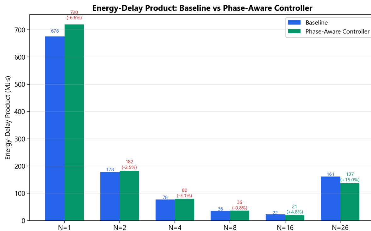
Figure 15: Energy-Delay Product (MJ-s), demonstrating a net energy-performance improvement of 14.85% for N = 26 and 4.75% for N = 16 , confirming the controller's effectiveness at operational computing scales.
