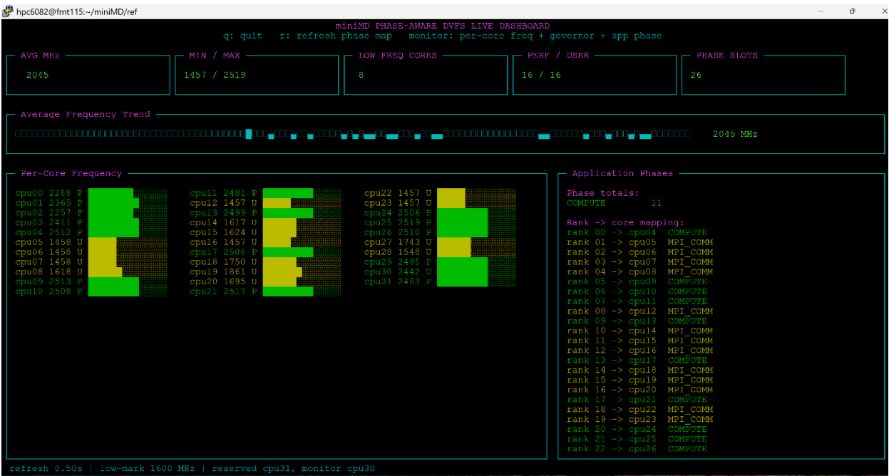
Figure 21: The miniMD Phase-Aware DVFS Live Dashboard in operation. The interface provides real-time telemetry of the frequency controller's actuation, showing per-core frequency levels (lower left), temporal average frequency trends (upper center below the 5 upper consecutive blocks), and the corresponding application phase hints retrieved from shared memory (lower right).
