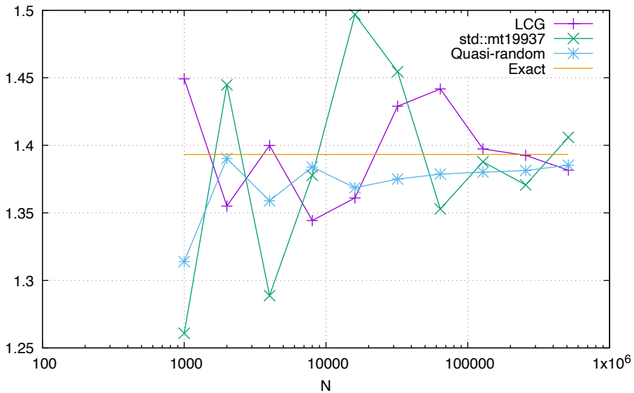
Integral estimate
