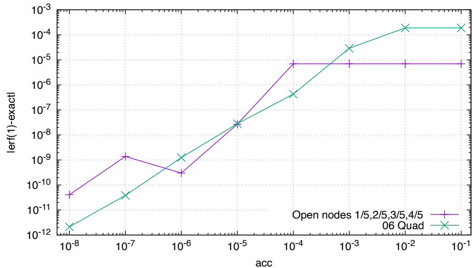
Convergence of erf(1) Comparison with Quad Homework
