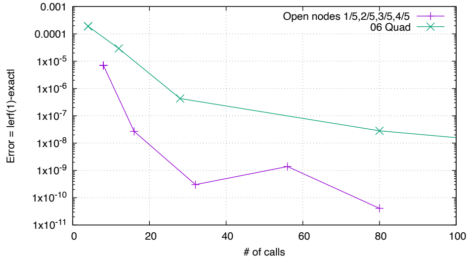
Error as a Function of # of calls (approx. of erf(1))
