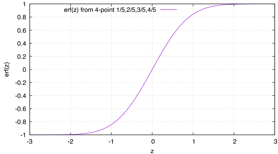
Error Function from the new 4-point integrator
