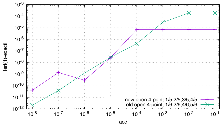
Convergence of erf(1) from the old- and new open 4-point nodes
