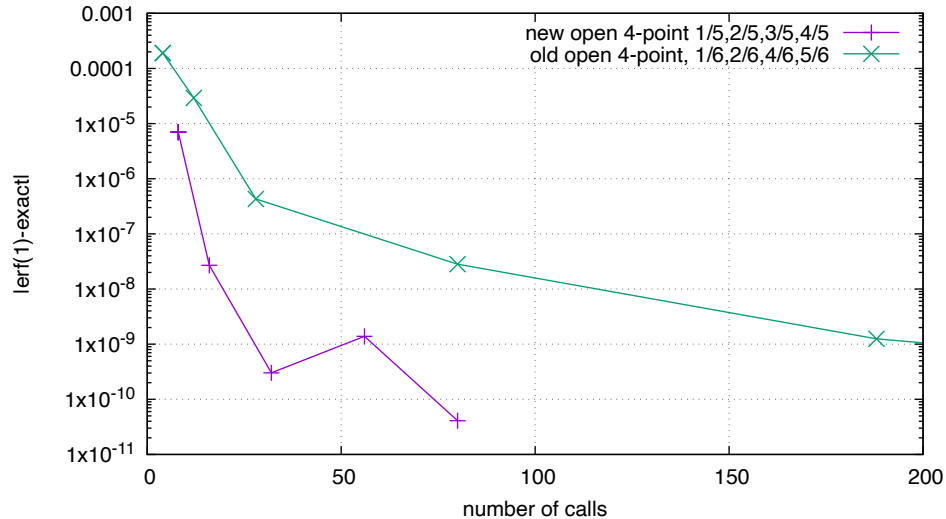
Convergence for erf(1)
