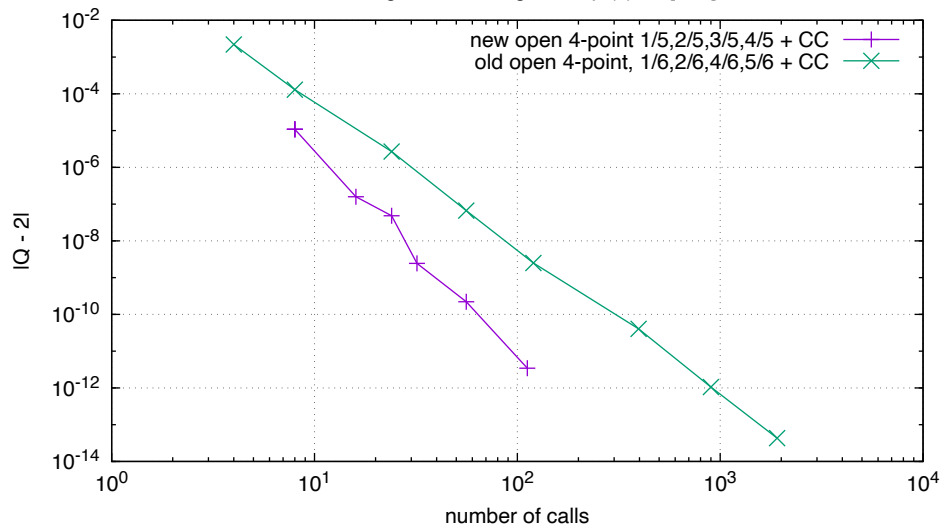
Convergence for integral 1/\sqrt{x} on [0, 1]
