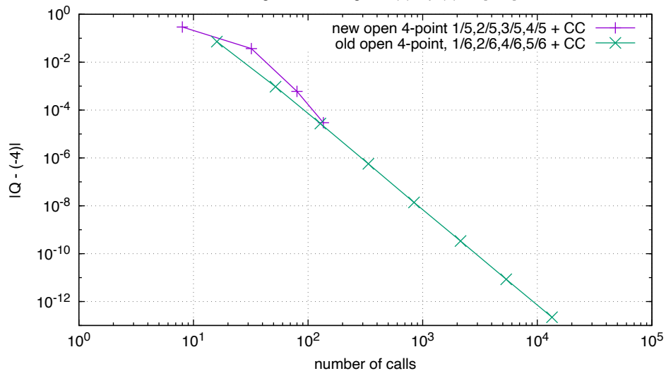
Convergence for integral \ln(x)/\sqrt{x} on [0, 1]
