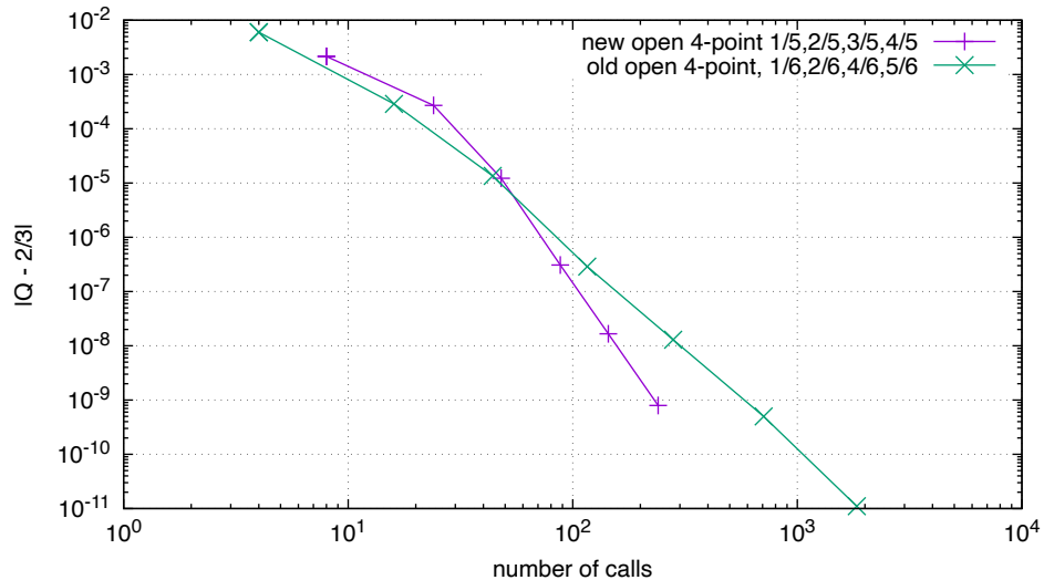
Convergence for integral \sqrt{x} on [0, 1]
