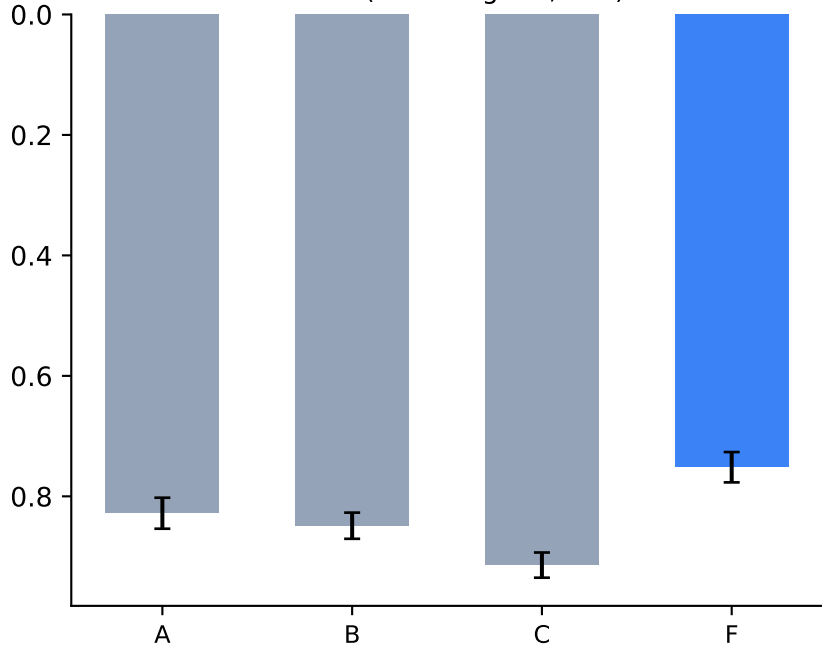
LTED \downarrow (class-aligned, aux)
