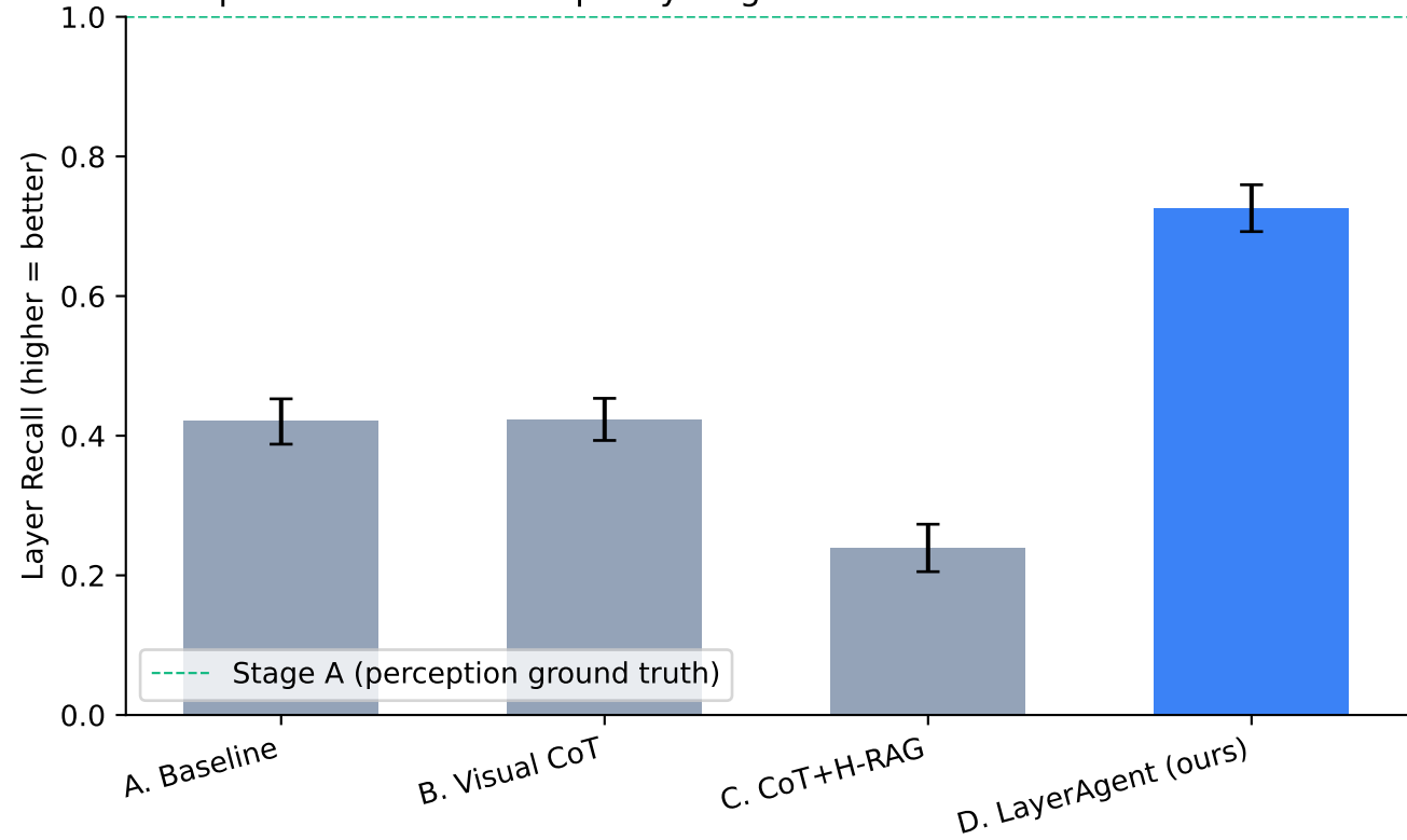
Perception-Generation Gap: LayerAgent recovers structure baselines miss
