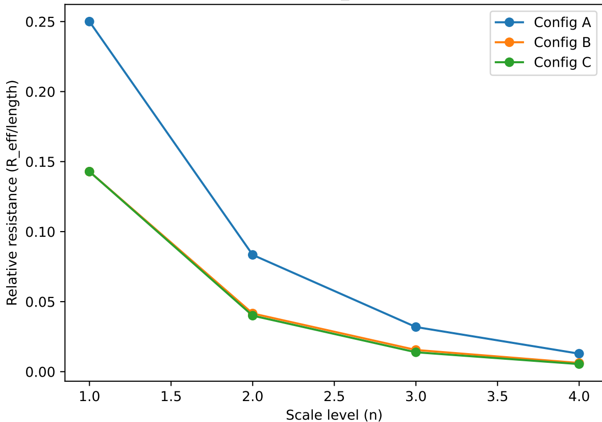
Relative resistance ( R_{\text{eff}}/\text{length} ) vs scale
