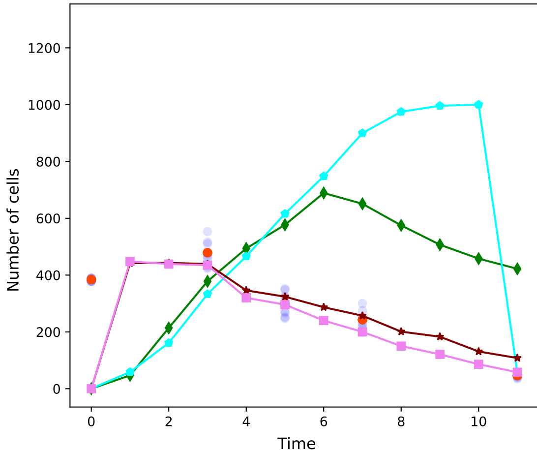
Number of cells in S/G2/Di phases
