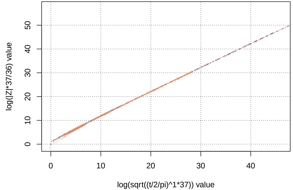
Figure 7: A graphical comparison for each investigated 1st degree L-function or Davenport-Heilbronn function of left column - \log(|Z_L|) vs \log(t) , right column - \log\left(|Z_L| \cdot \frac{N_C}{N_{\chi \neq 0}}\right) vs \log\left(\sqrt{\left(\frac{t}{2\pi}\right)^d \cdot N_C}\right) for top row - L(\chi_7(6, \cdot), 0.0 + I \cdot t) and bottom row - L(\chi_{37}(36, \cdot), 0.0 + I \cdot t) . With one conservative fitted model for extreme peak height trend growth rate.
