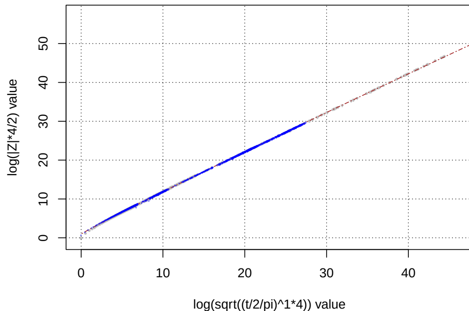
Growth behaviour of the s=0+It line largest L43 |Z| peaks log(|Z|*4/2) vs log(sqrt((t/2/pi)^1*4)) plot
