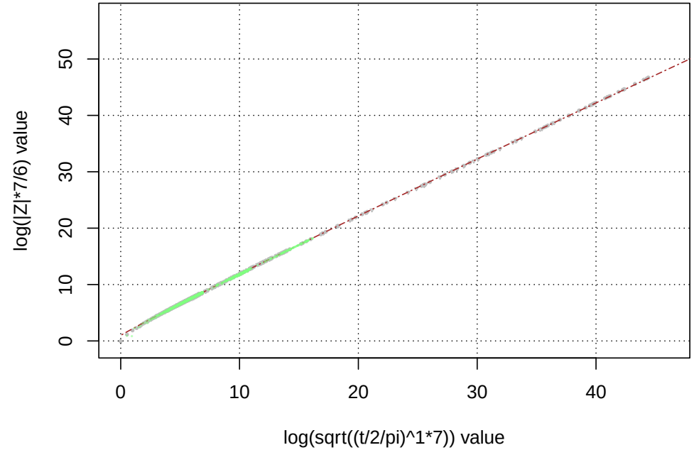
Growth behaviour of the s=0+It line largest L76 |Z| peaks log(|Z|*7/6) vs log(sqrt((t/2/pi)^1*7)) plot
