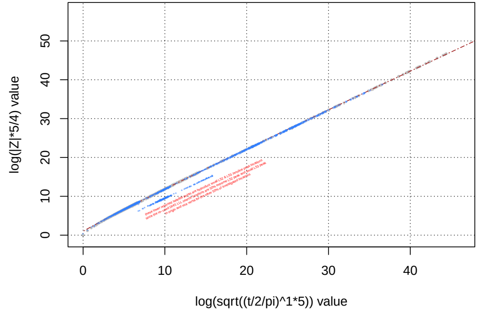
Figure 6: A graphical comparison for each investigated 1st degree L-function or Davenport-Heilbronn function of left column - \log(|Z_L|) vs \log(t) , right column - \log\left(|Z_L| \cdot \frac{N_C}{N_{\chi \neq 0}}\right) vs \log\left(\sqrt{\left(\frac{t}{2\pi}\right)^d \cdot N_C}\right) for top row - L(\chi_5(3, \cdot), 0.0 + I \cdot t) and bottom row - L(\chi_5(2, \cdot), 0.0 + I \cdot t) . With one conservative fitted model for extreme peak height trend growth rate.
