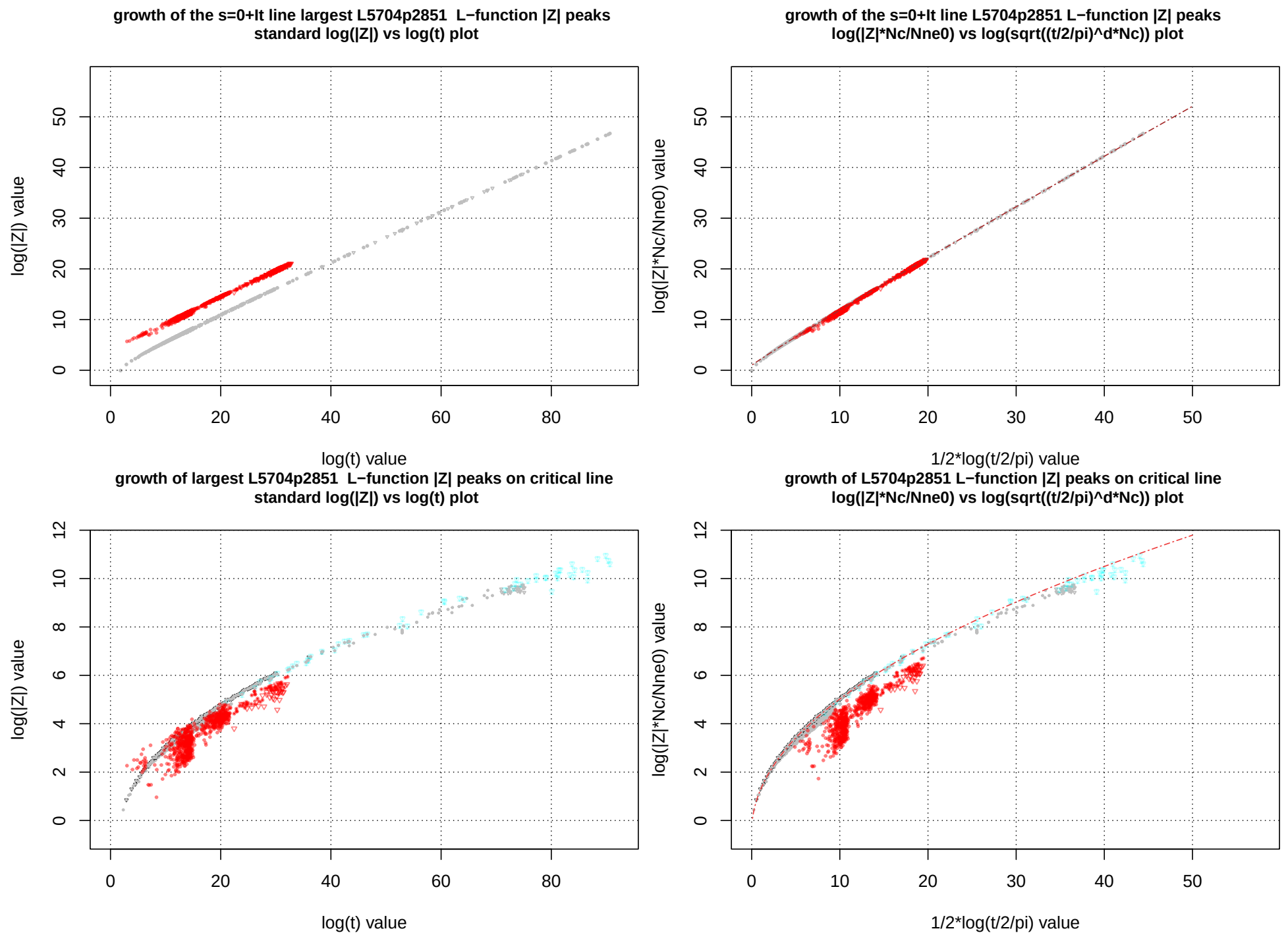
Figure 13: A graphical comparison for the L5704p2851 1st degree L-functions and the Riemann Zeta function extreme peaks of left panel - \log(|Z_L|) vs \log(t) , right panel - \log\left(|Z_L| \cdot \frac{N_C}{N_{x \neq 0}}\right) vs \log\left(\sqrt{\left(\frac{t}{2\pi}\right)^d \cdot N_C}\right) for top row - s = 0 + I \cdot t (zero line), and bottom row - s = 0.5 + I \cdot t (critical line). The x axis rescaling in the right panel is the same in figure 14 compared to figures 4-11. With one a different fitted model for extreme peak height trend growth rate depending on \text{Re}(s) . Riemann Zeta function behaviour shown in gray for known peak heights (and cyan for high t preliminary peak height estimates).
