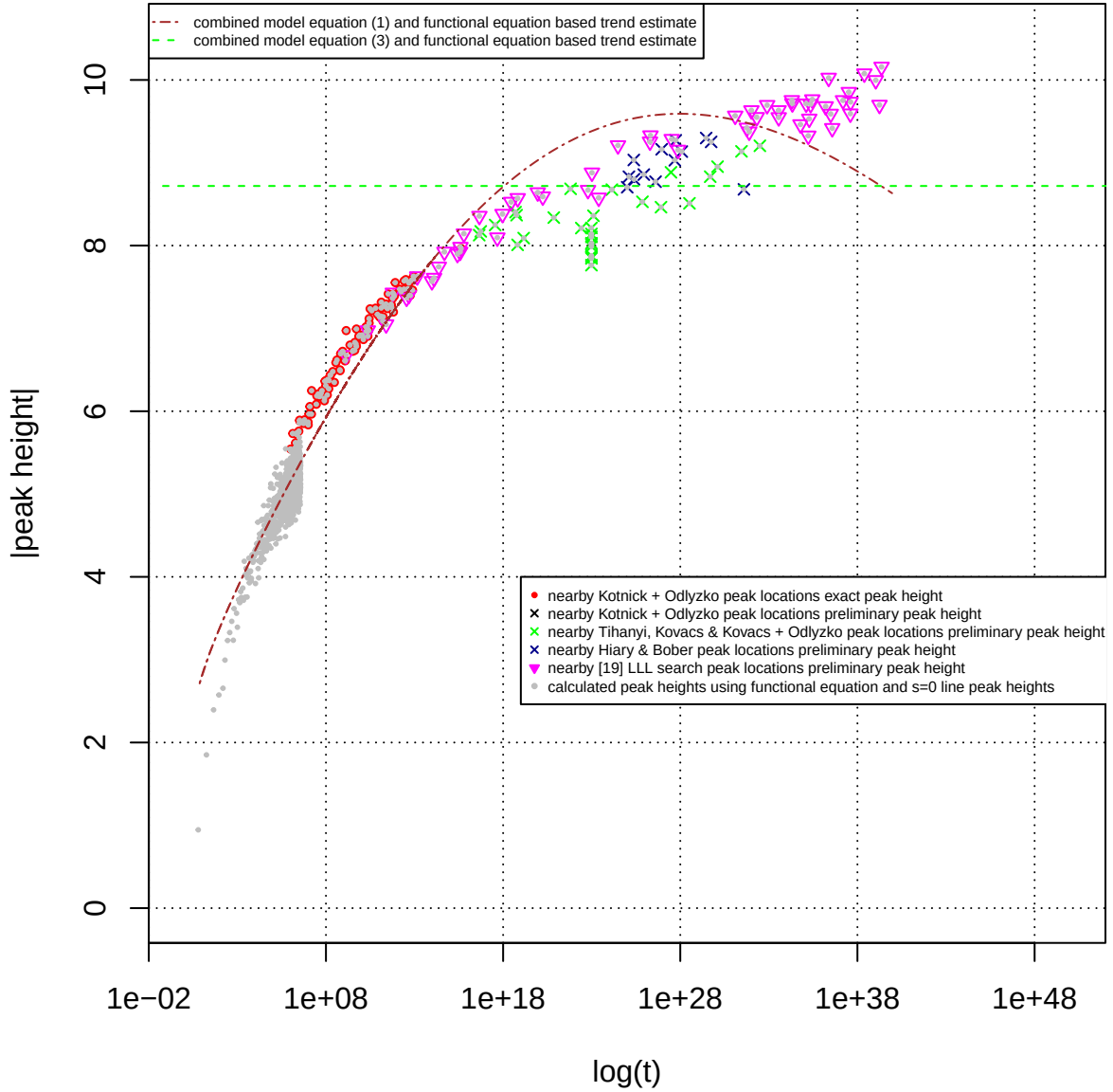
Figure 15: Observed |Z| versus \log(t) scatterplot of (i) good precision extreme Riemann Siegel Z function peak heights on the s = 1 + I \cdot t line between 1e6 < t < 1e13 (red solid circles) equation (16) and (ii) preliminary extreme Riemann Siegel Z function peak heights between 1e6 < t < 1e40 based on spectral filtered heavily truncated Euler products based approximation method (v) overlayed by (I) dot-dashed brown line and green dashed line of two mapped trend estimates based on fitted s = 0 + I \cdot t extreme peak behaviour (equations (1) and (3)) and the known functional equation and (II) shown as gray points s = 0 + I \cdot t extreme peak heights transformed by the known functional equation
