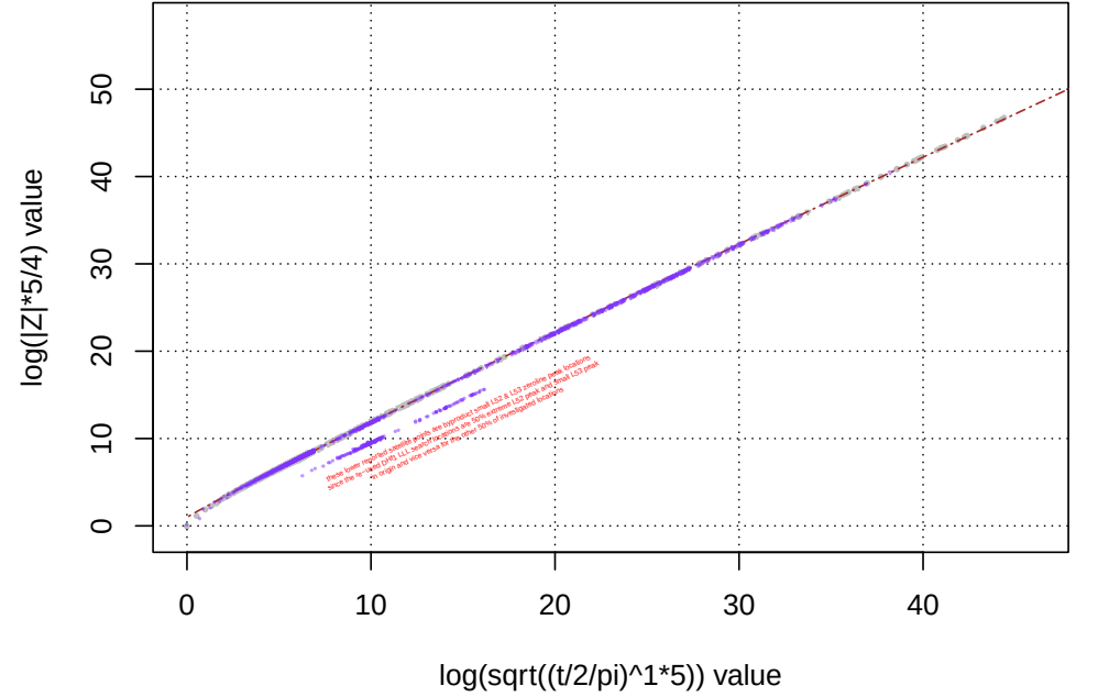
Growth behaviour of the s=0+It line largest L52 |Z| peaks log(|Z|*5/4) vs log(sqrt((t/2/pi)^1*5)) plot
