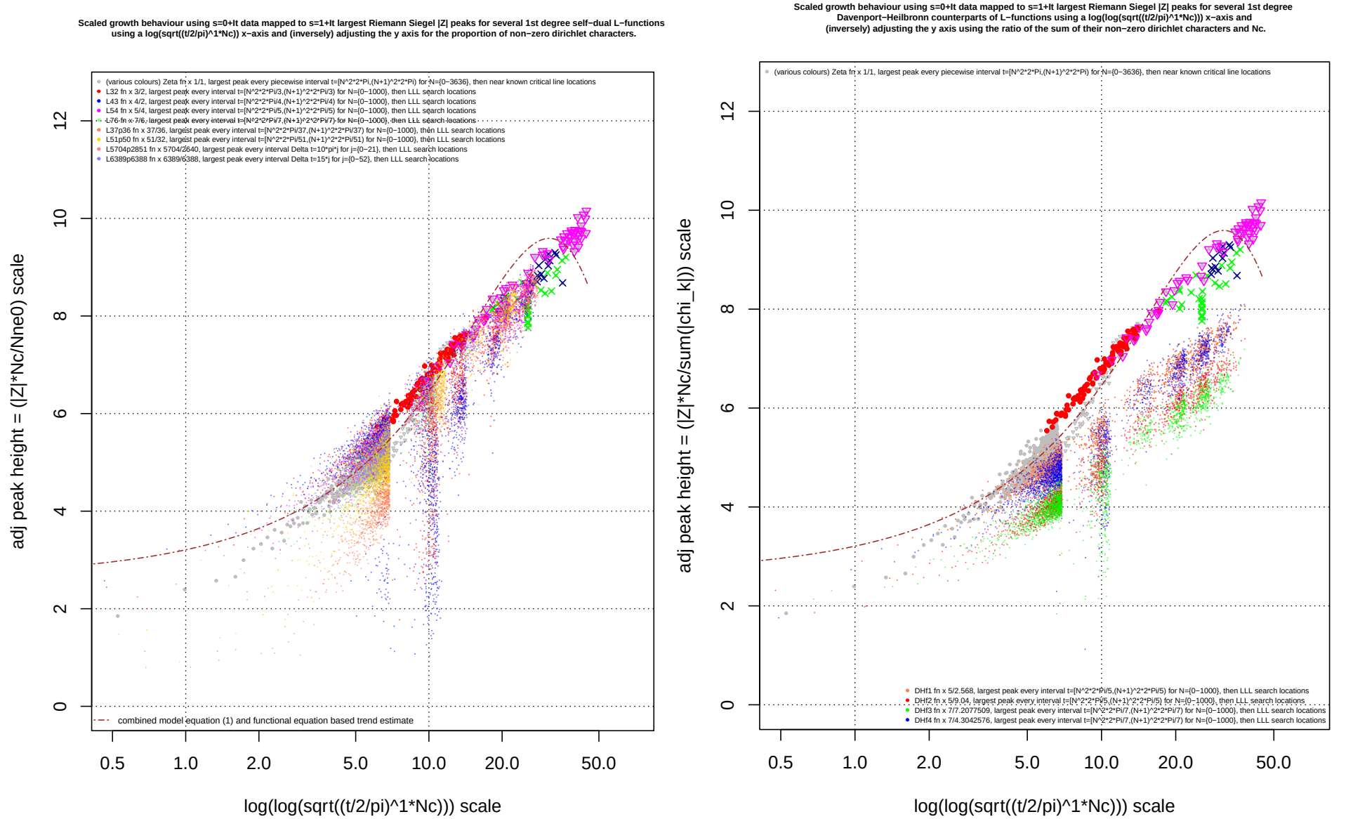
Figure 16: Rescaled XY axes overlay of the growth behaviour of extreme Riemann Siegel Z function peak heights |Z| for different 1st degree self-dual L-functions in the interval t < 1e30 mapped from the s = 0 + I \cdot t line to the s = 1 + I \cdot t line and compared to \zeta(1 + I \cdot t) extreme peak behaviour. The |Z| values on the Y axis are scaled by the ratio of the (L-function conductor value)/(number of non-zero dirichlet characters mod N_C ) i.e. \log(|Z| \cdot \frac{N_C}{N_{\chi \neq 0}}) . (For the n-periodic Davenport-Heilbronn functions \log(|Z| \cdot \sum_{k=1}^n \frac{1}{|X_k|}) (where n=5,7 for the investigated self-dual D-H functions in this paper) is used for Y axis rescaling.) The X axis is transformed by the first quiescent region value of the L-function and hence the displayed scale is \log(\log(\sqrt{(\frac{t}{2\pi})^1 \cdot N_C})) .
