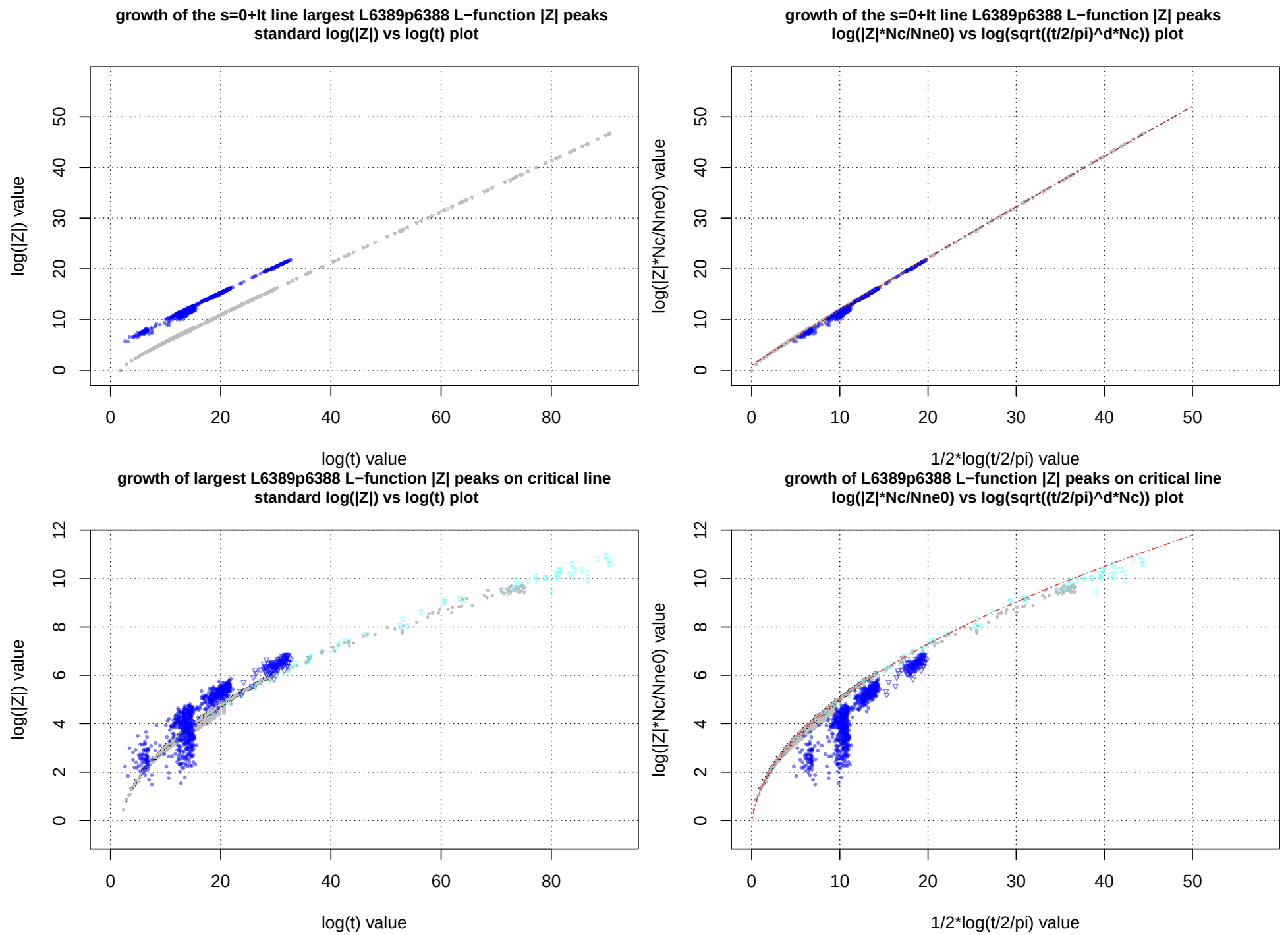
Figure 14: A graphical comparison for the L6389p6388 1st degree L-functions and the Riemann Zeta function extreme peaks of left panel - \log(|Z_L|) vs \log(t) , right panel - \log\left(|Z_L| \cdot \frac{N_C}{N_{x \neq 0}}\right) vs \log\left(\sqrt{\left(\frac{t}{2\pi}\right)^d \cdot N_C}\right) for top row - s = 0 + I \cdot t (zero line), and bottom row - s = 0.5 + I \cdot t (critical line). The x axis rescaling in the right panel is the same in figure 15 compared to figures 4-11. With one a different fitted model for extreme peak height trend growth rate depending on \text{Re}(s) . Riemann Zeta function behaviour shown in gray for known peak heights (and cyan for high t preliminary peak height estimates).
