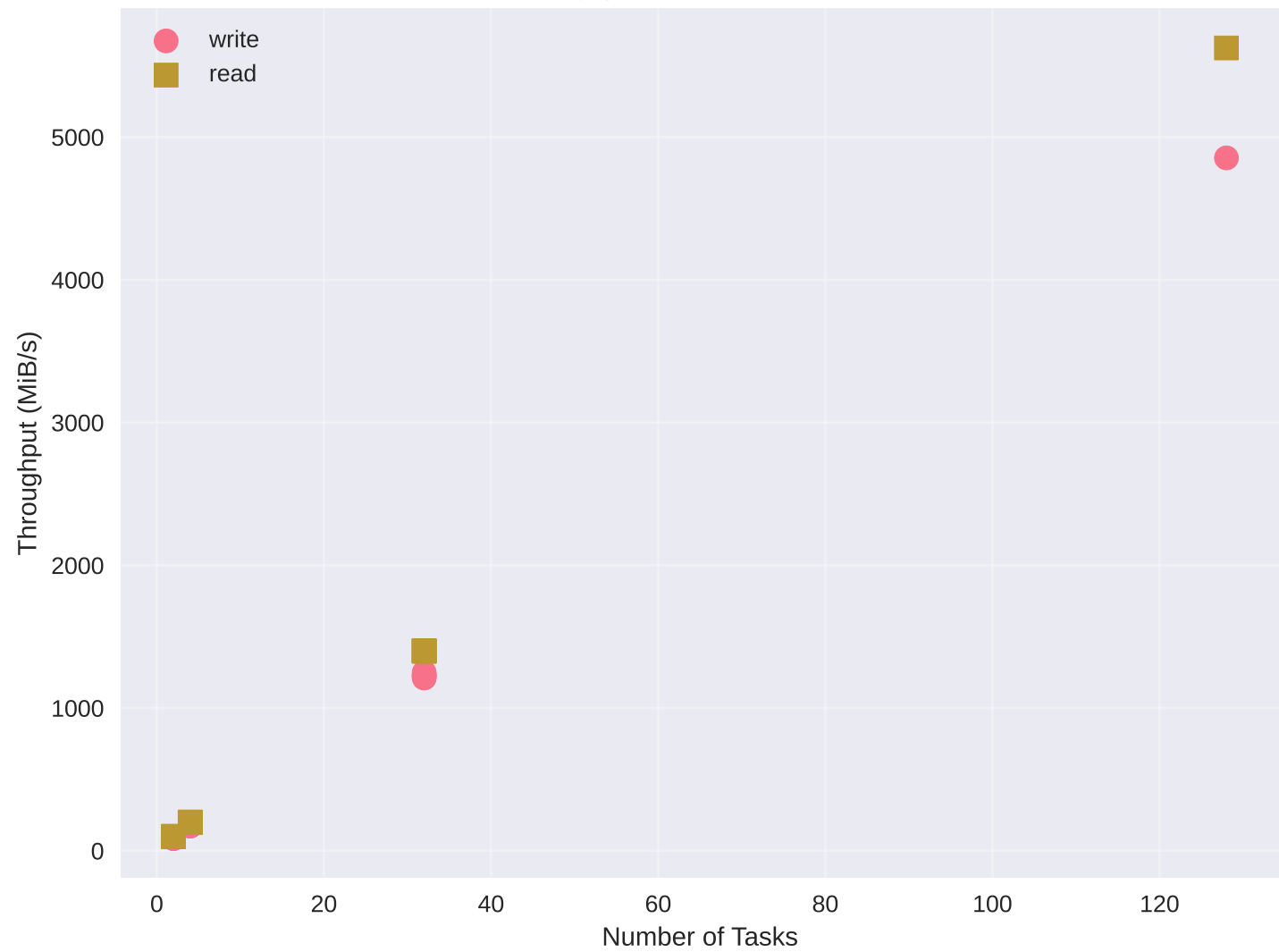
Throughput vs Number of Tasks
