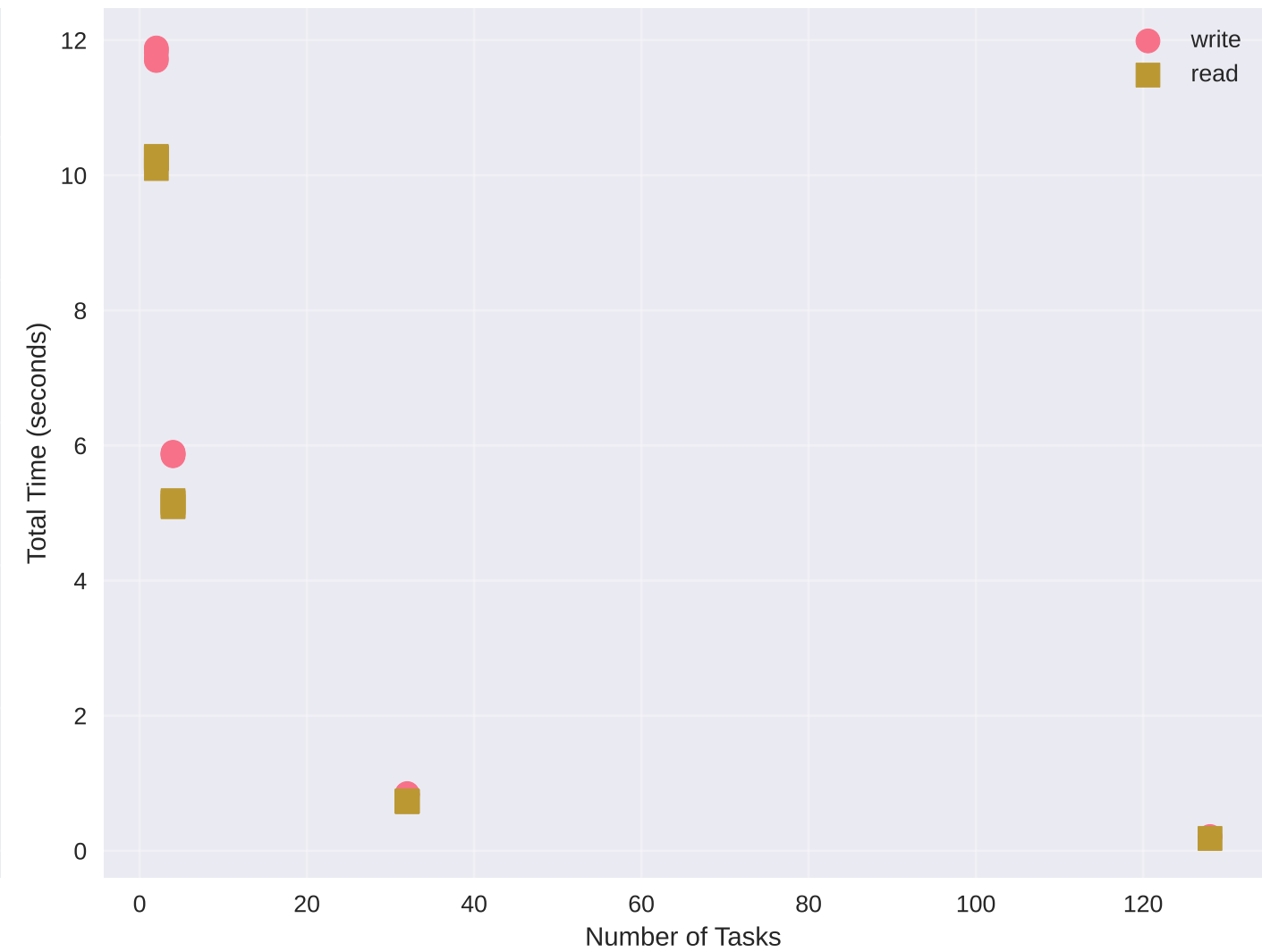
Total Time vs Number of Tasks
