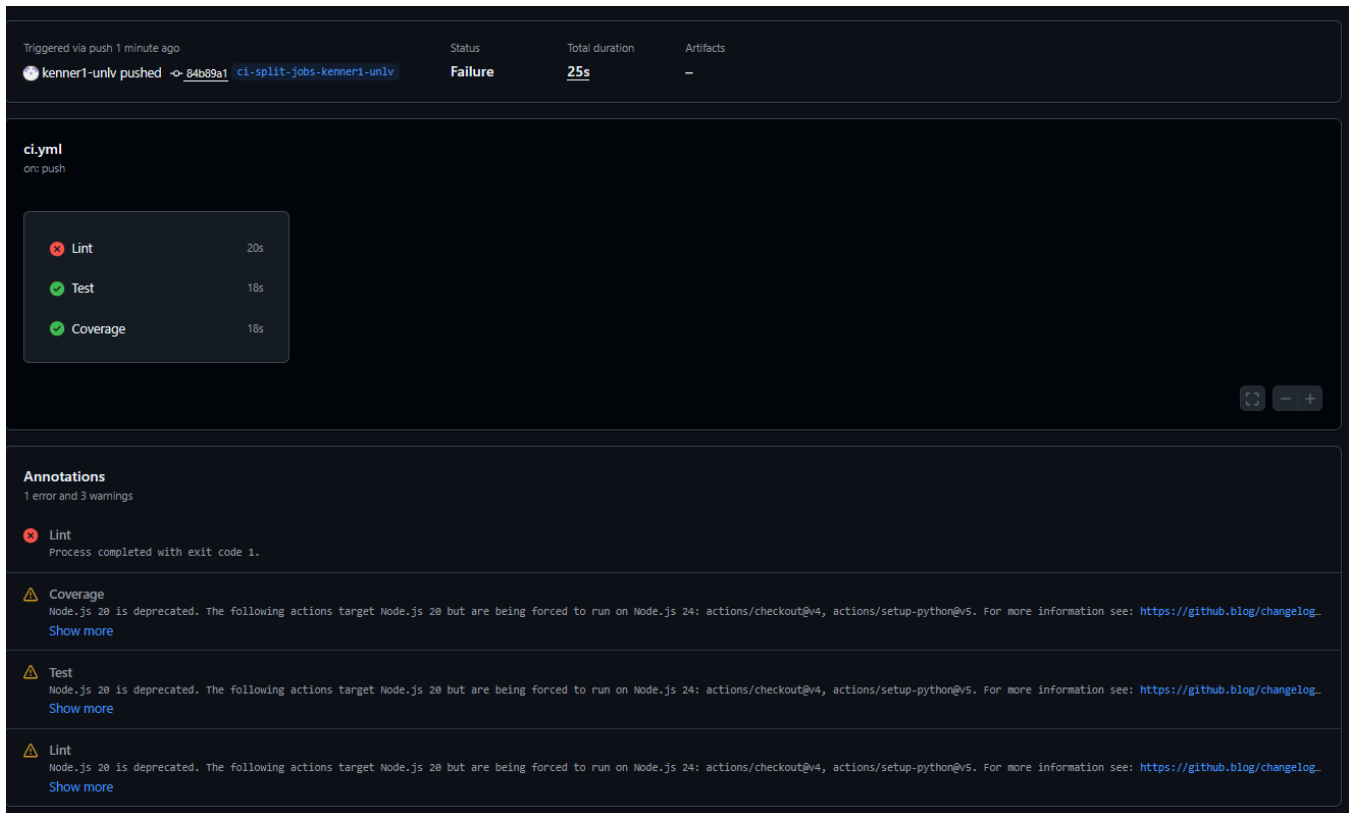
Figure 12. Controlled failure run #22: Lint is red while Test and Coverage remain green.
