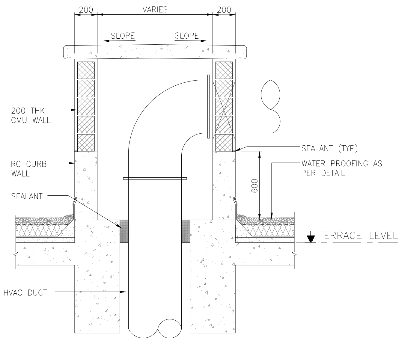
ROOF DUCT OPENING DETAIL
