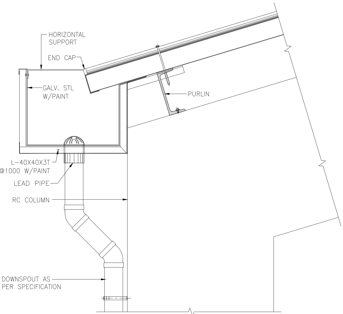
TYPICAL SECTION FOR RAIN GUTTER DETAIL AND DOWN SPOUT
