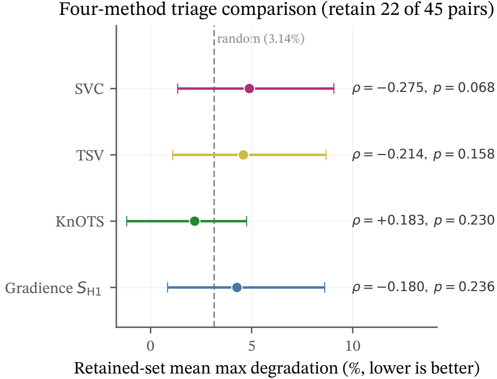
Figure 3: Four-method triage comparison on the 45 evaluated cross-task pairs. Methods are ordered by magnitude of Spearman \rho between their risk score and max degradation. Horizontal error bars are family-pair-blocked bootstrap 95% CIs on the retained-set mean. Vertical dashed line: random-baseline mean max degradation (3.14%) across all 45 pairs. Per-method \rho and p are annotated inline. No method’s CI excludes the random baseline. Three of four methods sit visibly to the right of baseline (worse than random on retained-set mean degradation); KnOTS alone sits to the left with a right-signed \rho , but its CI crosses baseline.
