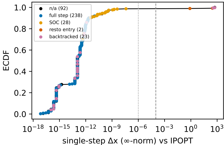
14 nav instances, 383 injected steps
