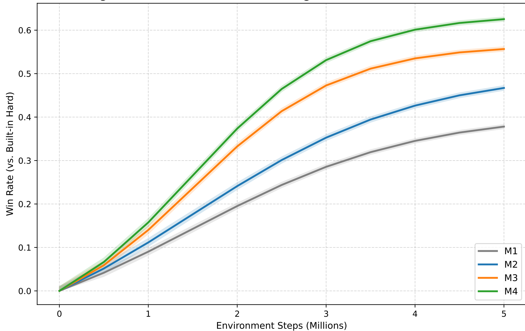
Figure 7: Multi-Seed 11v11 Learning Curves (10 Seeds, 95% CI)
