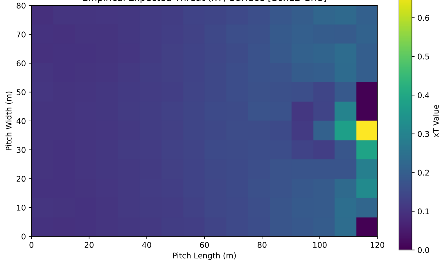
Empirical Expected Threat (xT) Surface [16x12 Grid]
