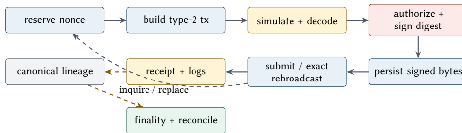
Figure 5. EVM transaction, replacement, observation, and reconciliation lifecycle.
