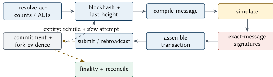
Figure 6. Solana message lifetime, signing, commitment, and reconciliation lifecycle.
