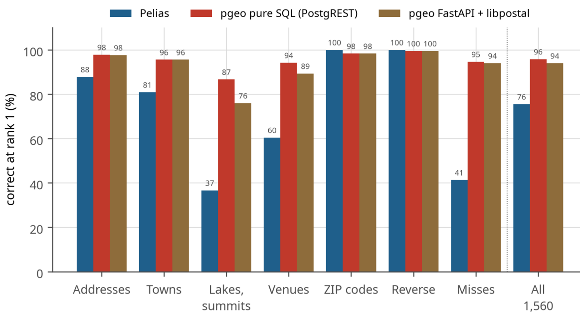
Figure 7. Correct answers by category. pgeo leads in every category except ZIP codes and reverse geocoding, where both engines are near perfect.
