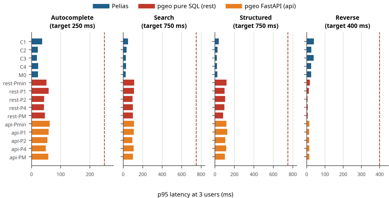
Figure 12. p95 latency per endpoint at 3 users for each configuration, against its target (dashed).
